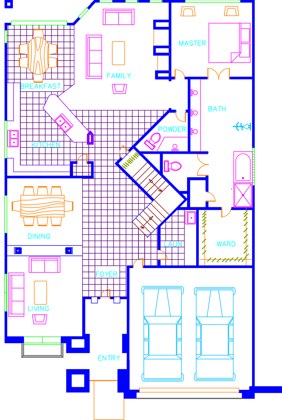
EXERCISE 11-6 HOUSE FLOOR PLAN SCALE 1/8" = 1'-0" LOWER LEVEL PAUL STEPHEN FUQUA 6/27/05
